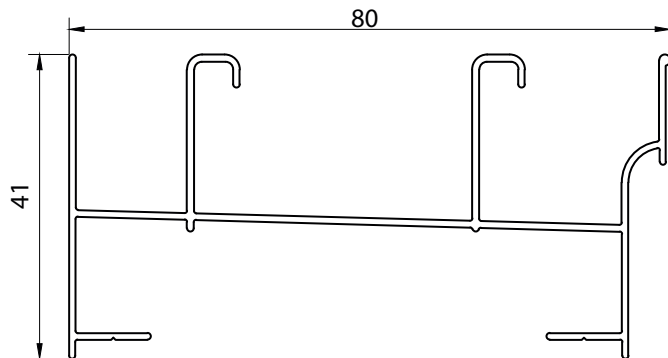
100 - MARCO CORREDIZA LIVIANO - PESO: 0.584 KG x Mts.
